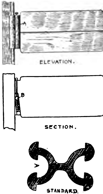
FIG. 42.—Brackets and Standard of Smith's Adjustable Shelving (Section 188).
